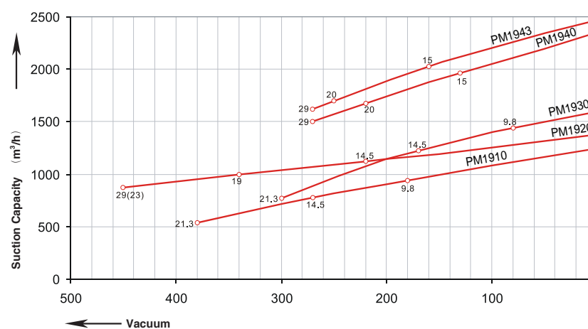
Vacuum Selection diagram 60Hz
